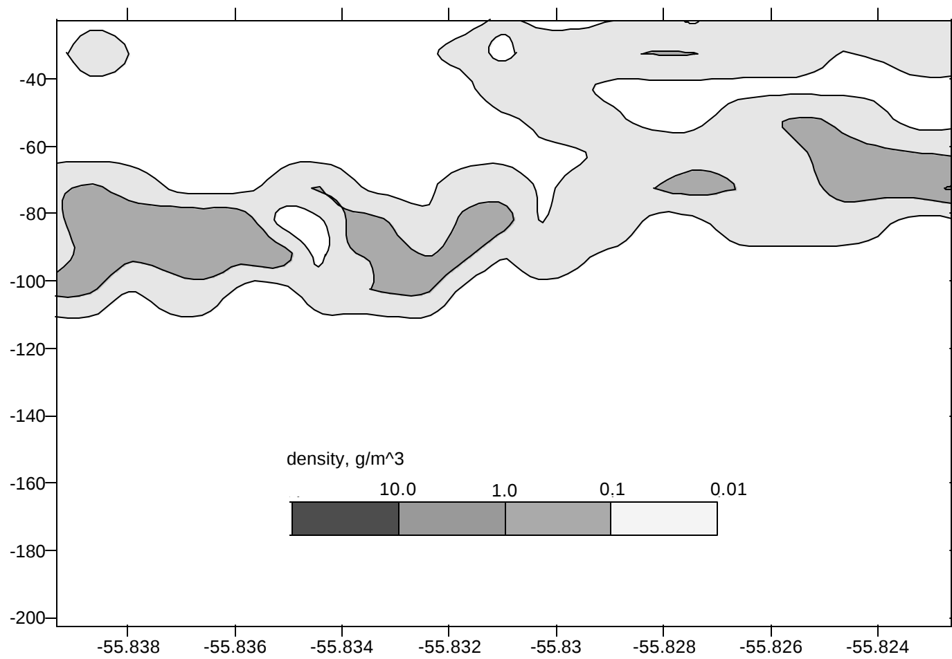
Fig 8. Krill biomass vertical distribution over horizontal distance of the daytime trawling 48. Further detail as in Fig.4. Net density is zero. Mean acoustic density is 32 \text{g}/1000\text{m}^3 .
