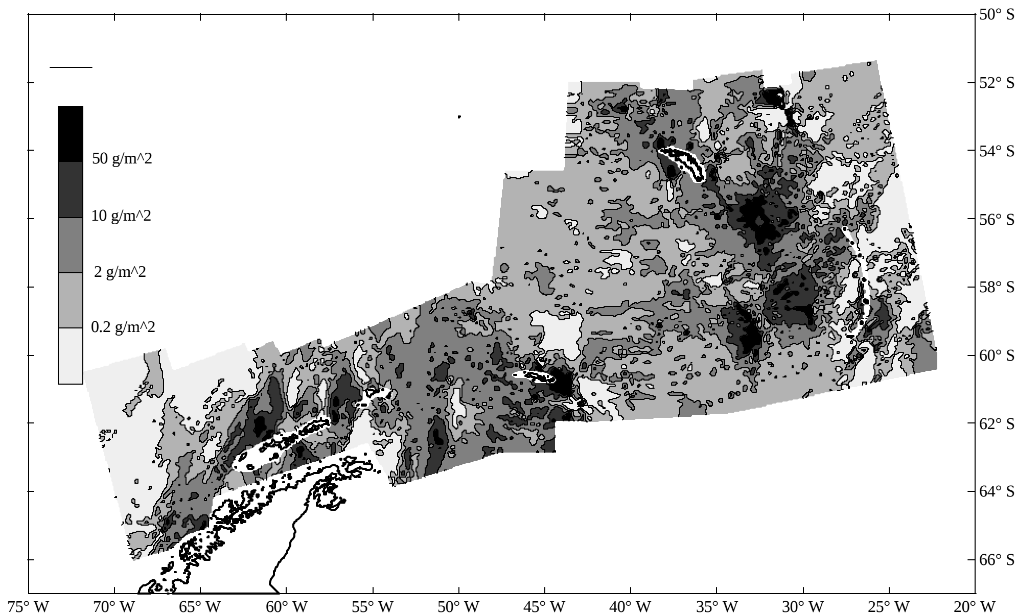
Fig. 11. Krill acoustic density distribution based on the results of the CCAMLR-2000 Synoptic Survey of Scotia Sea.
