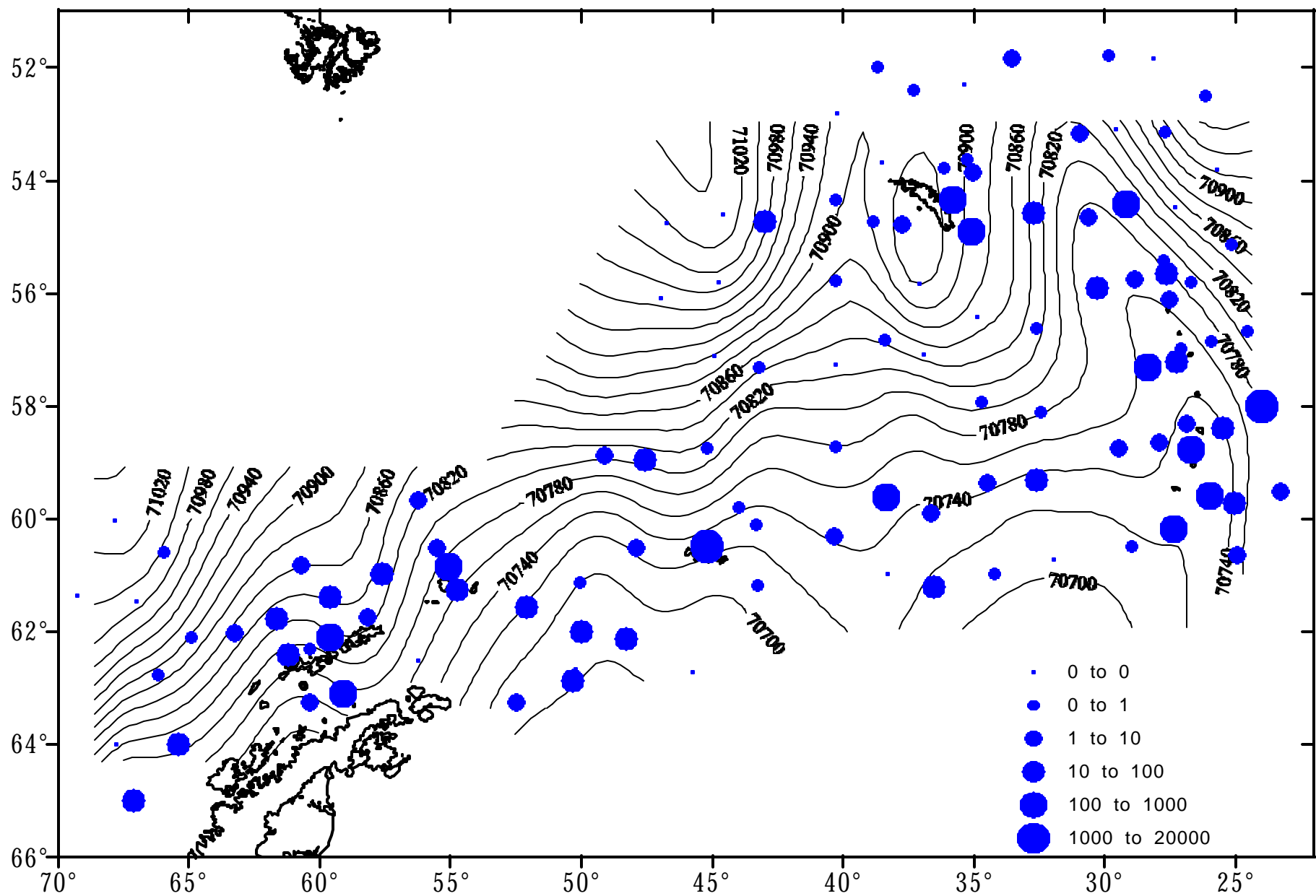
Fig. 10. Distribution of krill density ( \text{g/m}^2 ) obtained from trawl samples during the CCAMLR-2000 Synoptic Survey of Scotia Sea.
