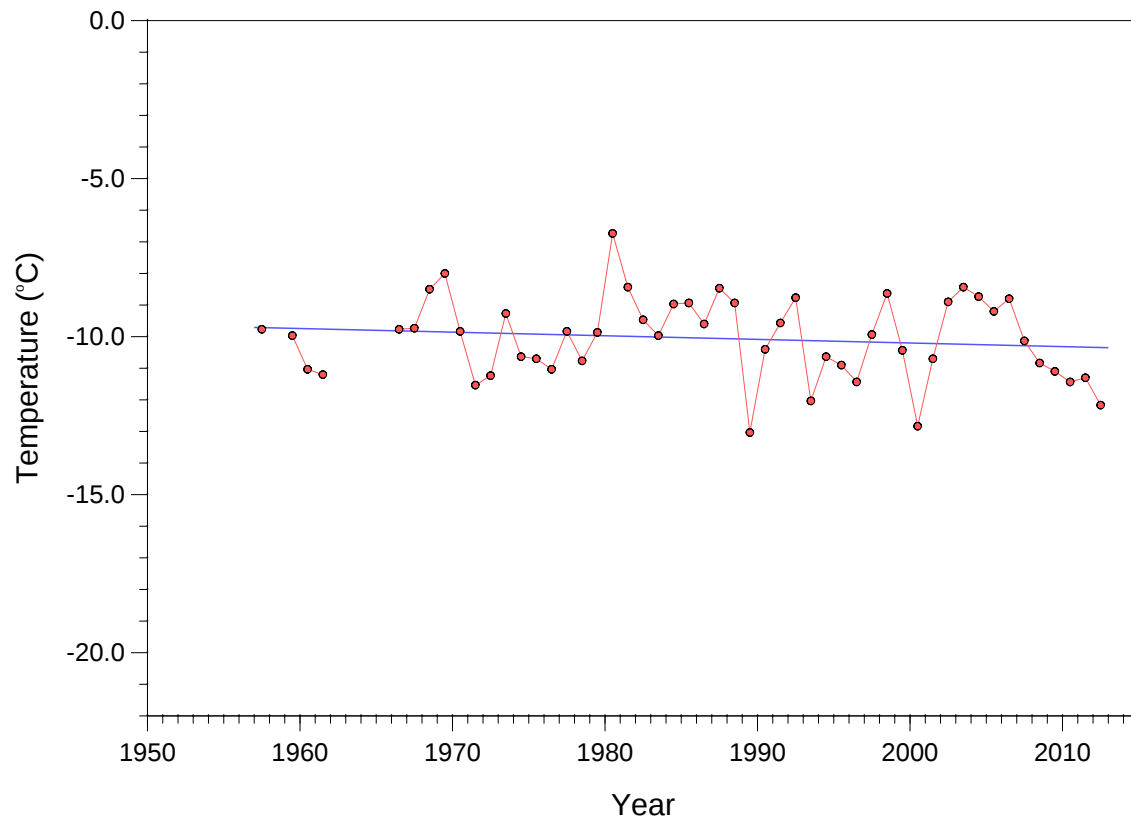
Autumn (MAM) surface temperature
