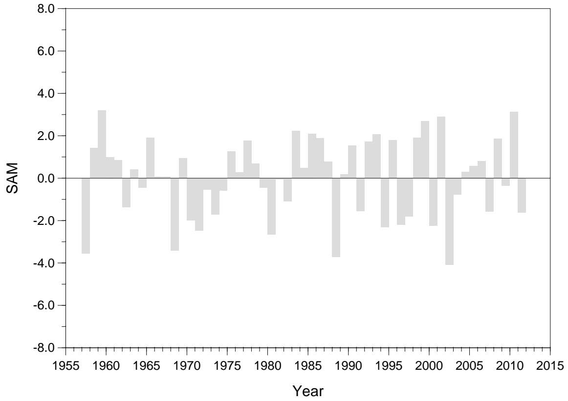
SAM Index: Spring (SON)
