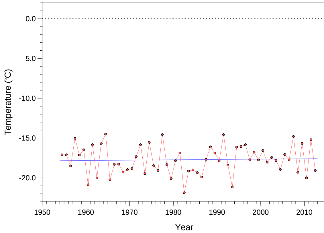
Winter (JJA) surface temperature
