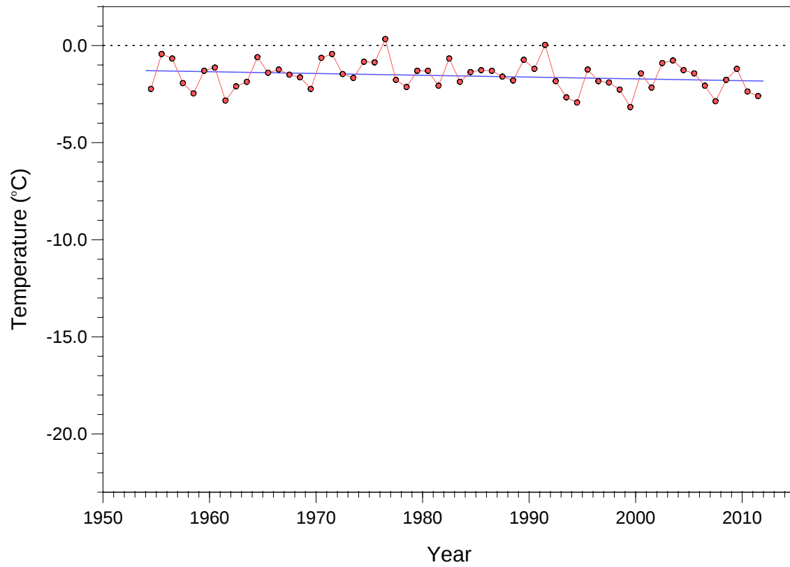
Summer (DJF) surface temperature
