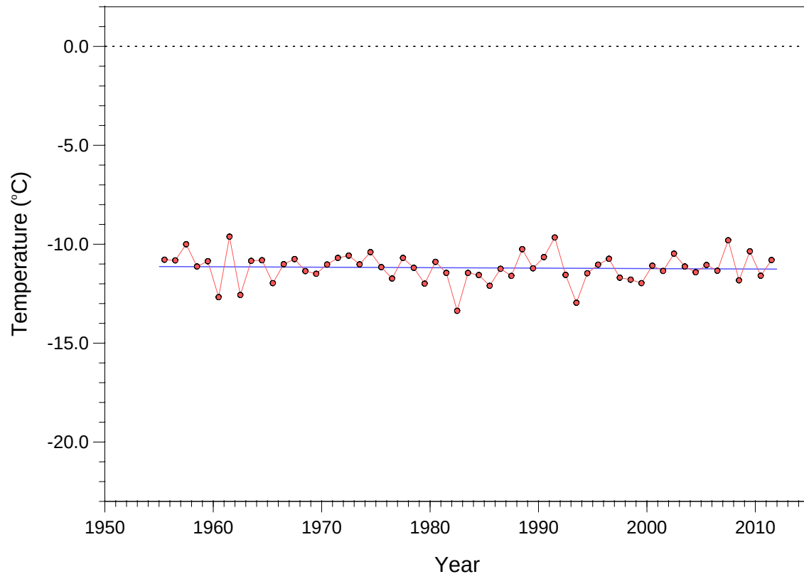
Annual surface temperature
