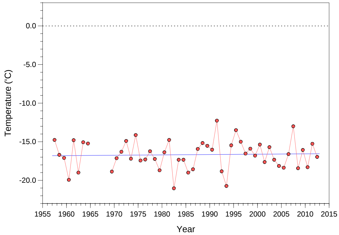
Winter (JJA) surface temperature
