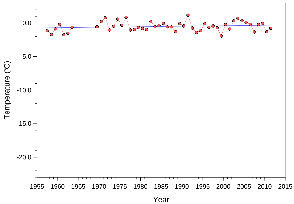
Summer (DJF) surface temperature
