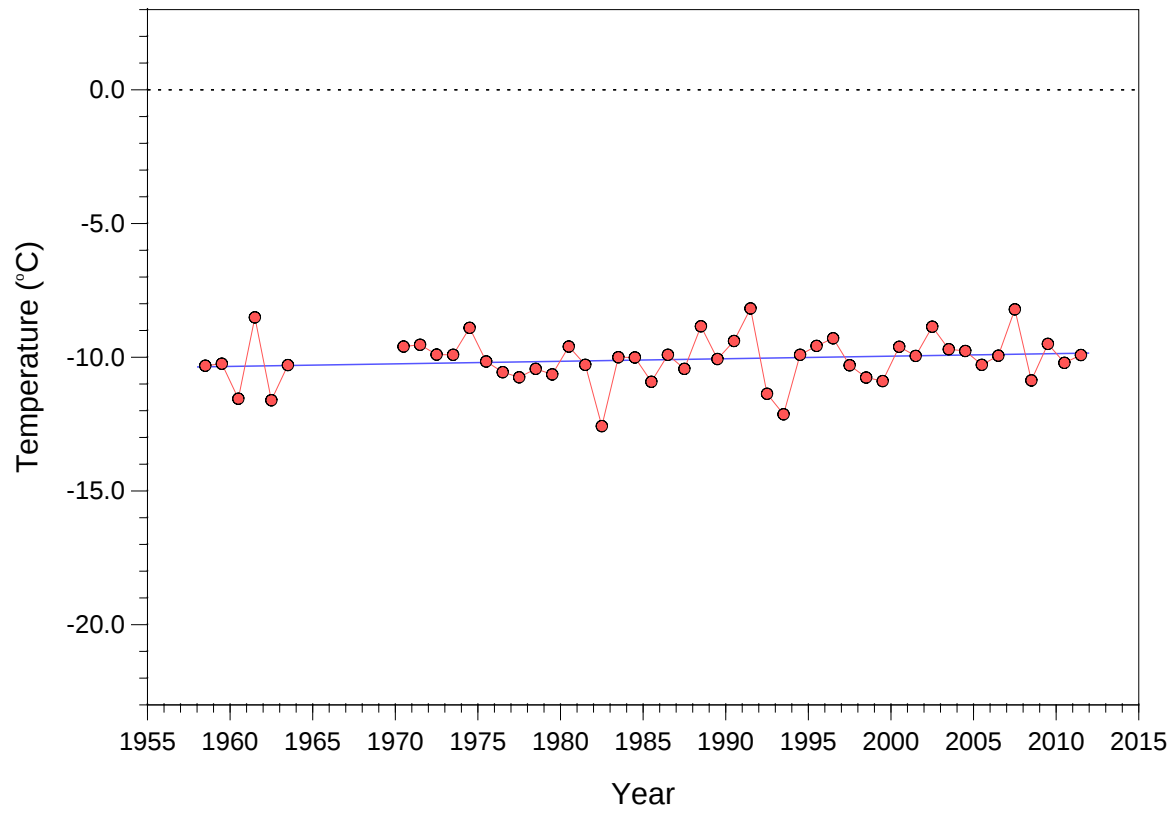
Annual surface temperature
