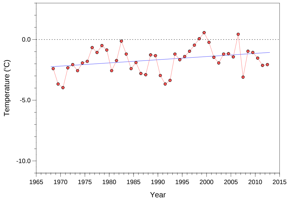
Autumn (MAM) surface temperature
